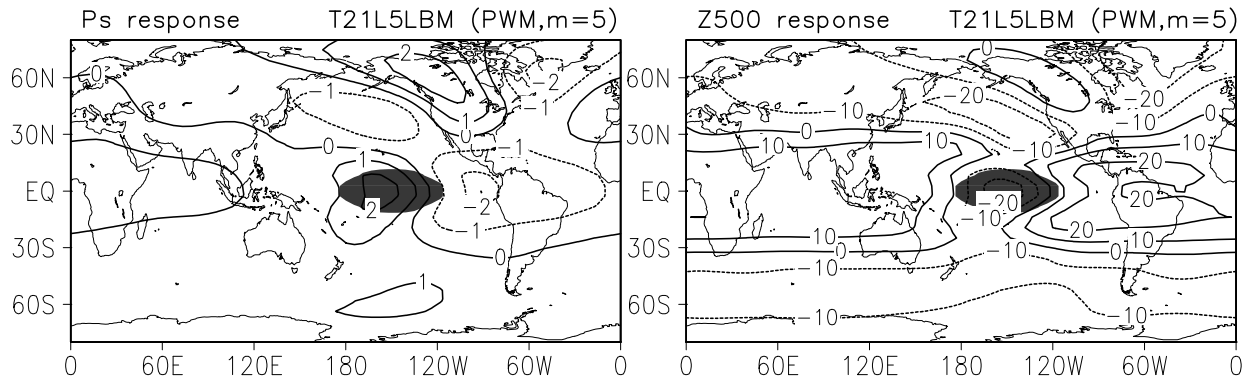
Figure 3.3 Example of the T21L5 linear response using PWM. Surface pressure (left) and 500 hPa geopotential height (right). Shading denotes a heating at \sigma = 0.44 ( Q \geq 1\text{K day}^{-1} ).
