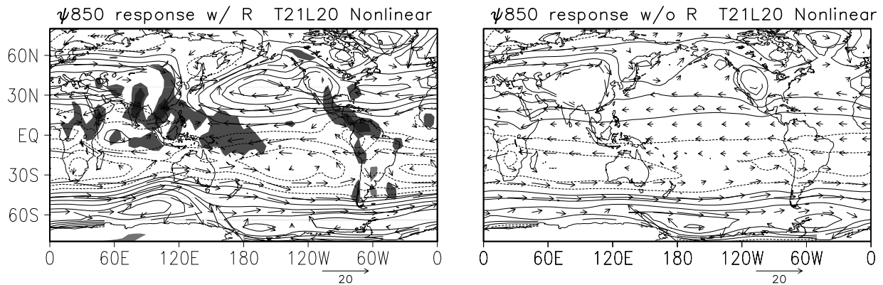
Figure 6.1 Example of the T21L20 nonlinear integration represented by 850 hPa stream function (contour) and wind (vector) averaged for days 15–25. The left (right) panel shows responses with (without) residual forcing R . The vertically averaged heating due to R is denoted by shading in the left panel. Note that both integrations are initialized by a zonally uniform state.
