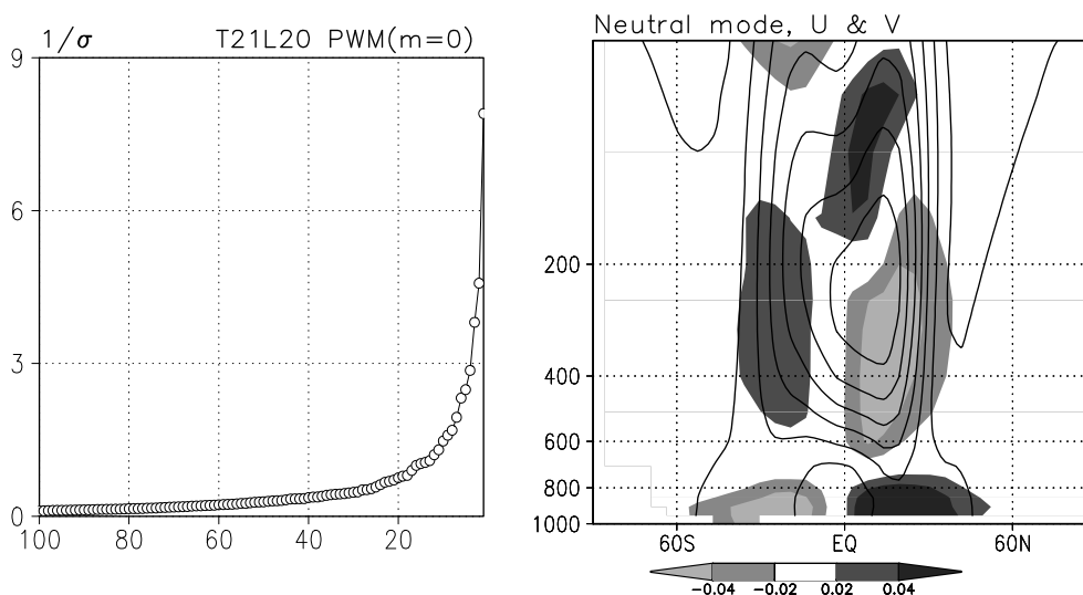
Figure 5.1 Example of singular vector analysis to zonal mean components of the T21L20 PWM. Inverse singular value for leading 100 modes (left) and structure of the leading mode ( u : contour, v : shading). The horizontal (vertical) axis of the left panel corresponds to number of mode (time scale of unit 1 \times 10^{11} \text{ s}^{-1} ).
