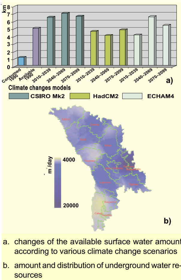
Figure 5.9 Water reserves of the Republic of Moldova (surface and underground) and the modification of the available amount of surface water
